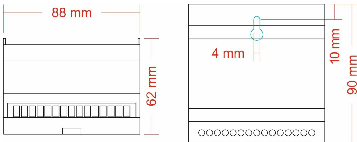
Mounting Drawing
