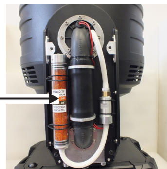
Silica gel desiccant in tube in the fixture head
