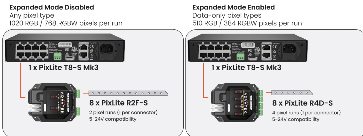
Figure 16: Connecting Receivers to Transmitter
