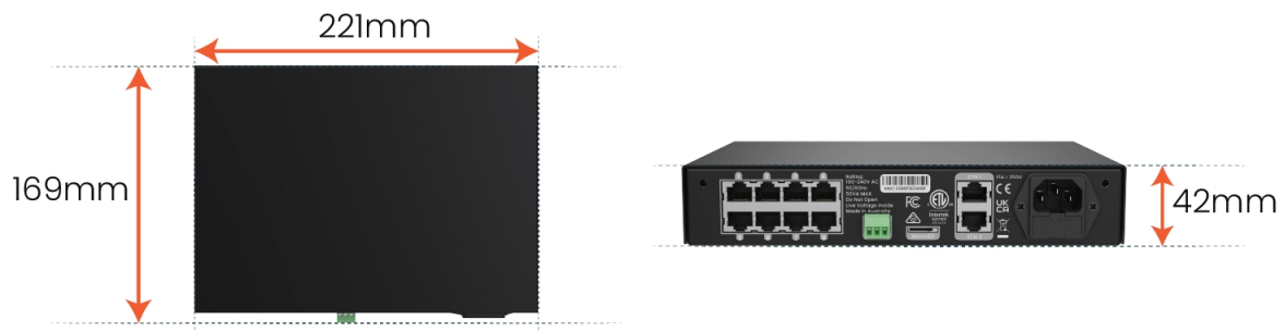
Figure 20: Mechanical Specifications
