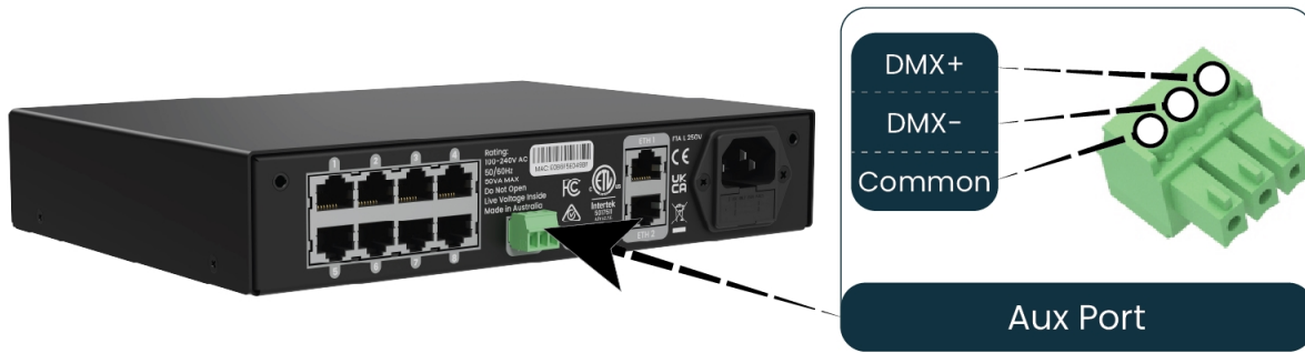
Figure 17: Location and Pinout of the Aux Port
