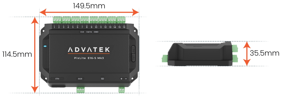
Figure 16: Mechanical Specifications
