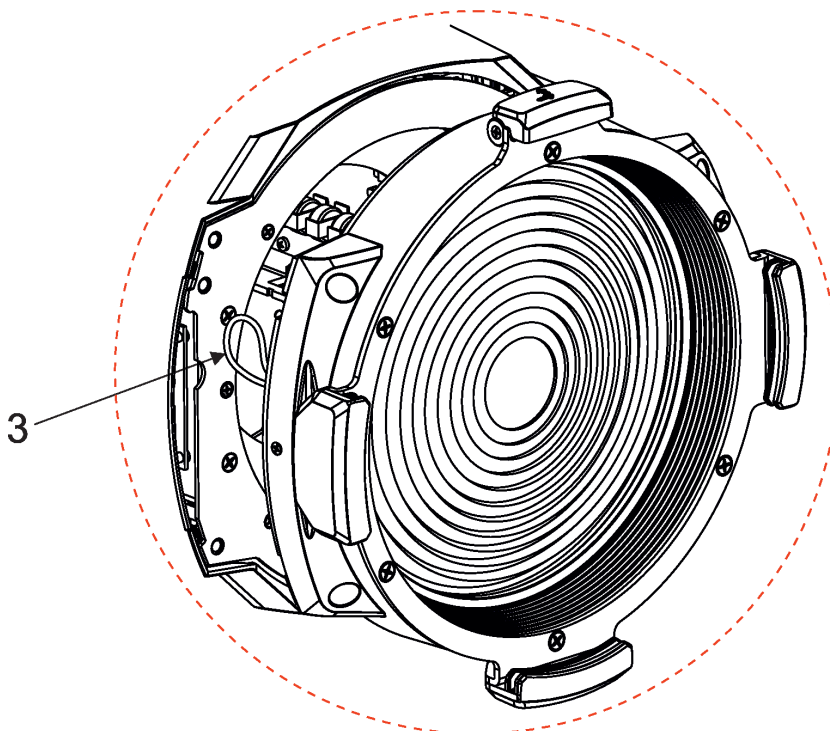
Detail A
