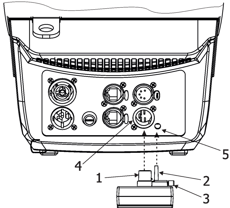
ROBE Wireless DMX/RDM Module
