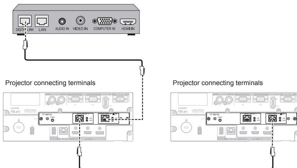
Example of twisted-pair-cable transmitter
