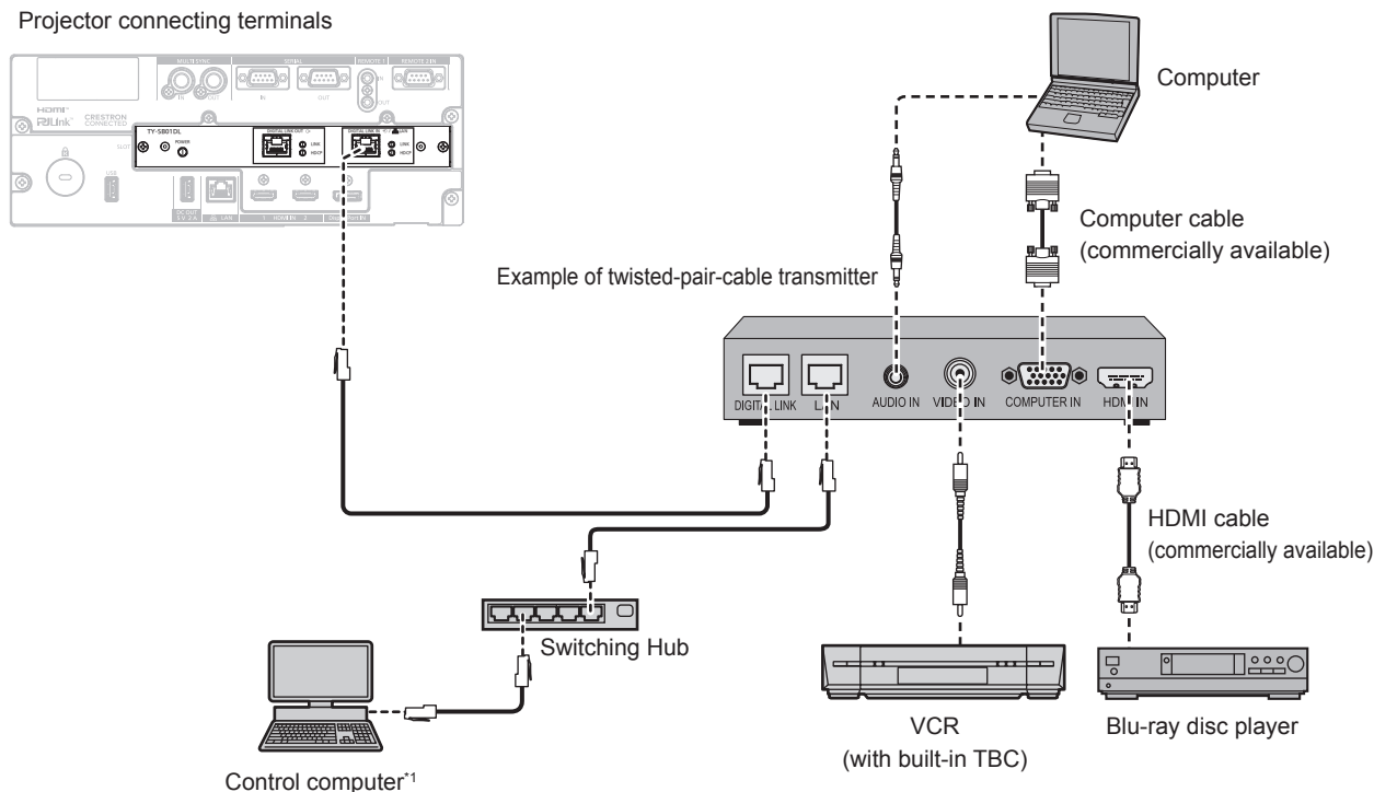
Projector connecting terminals
