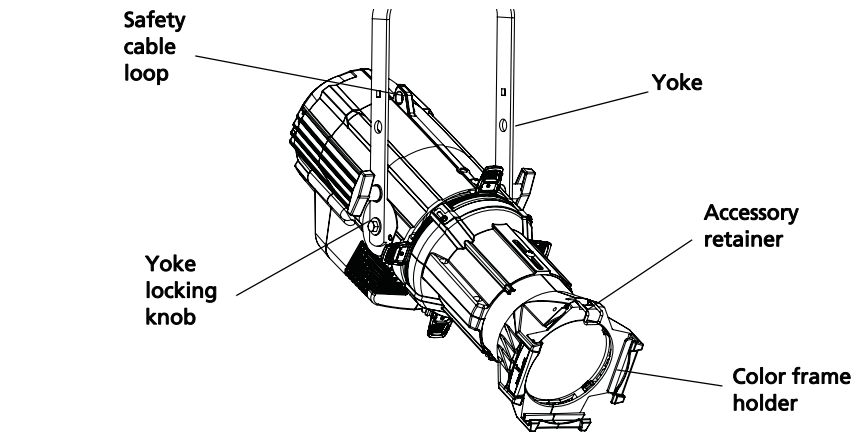
Figure-1.1 Components of the Source Four LED Profile fixture
