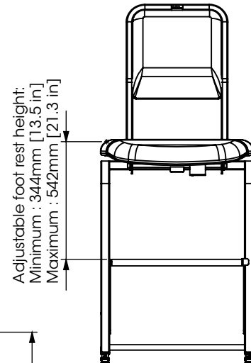
Fully adjustable Conductor's Chair
