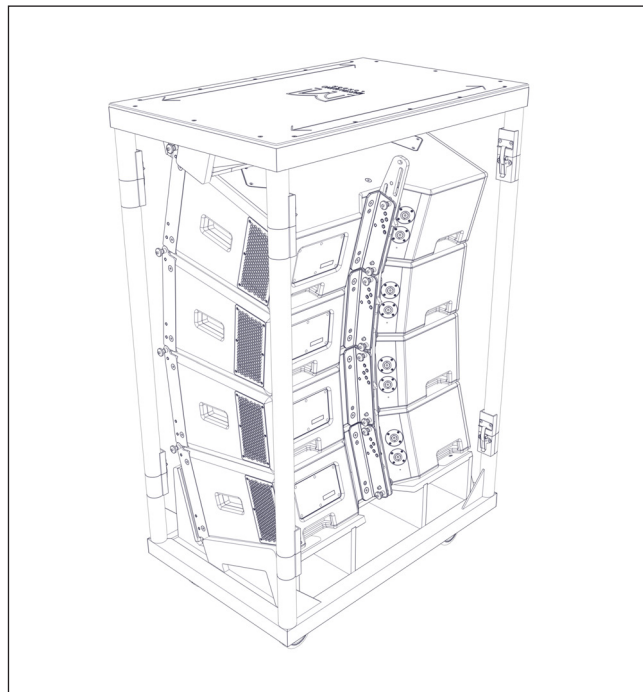
Fig. 7 - transport cart
