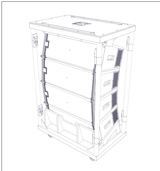
Fig 6 - transport cart
