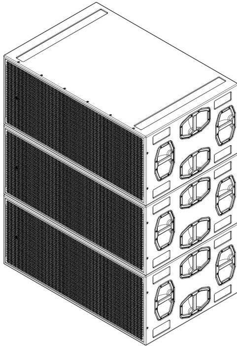
Standard subwoofer column All subwoofers forward
