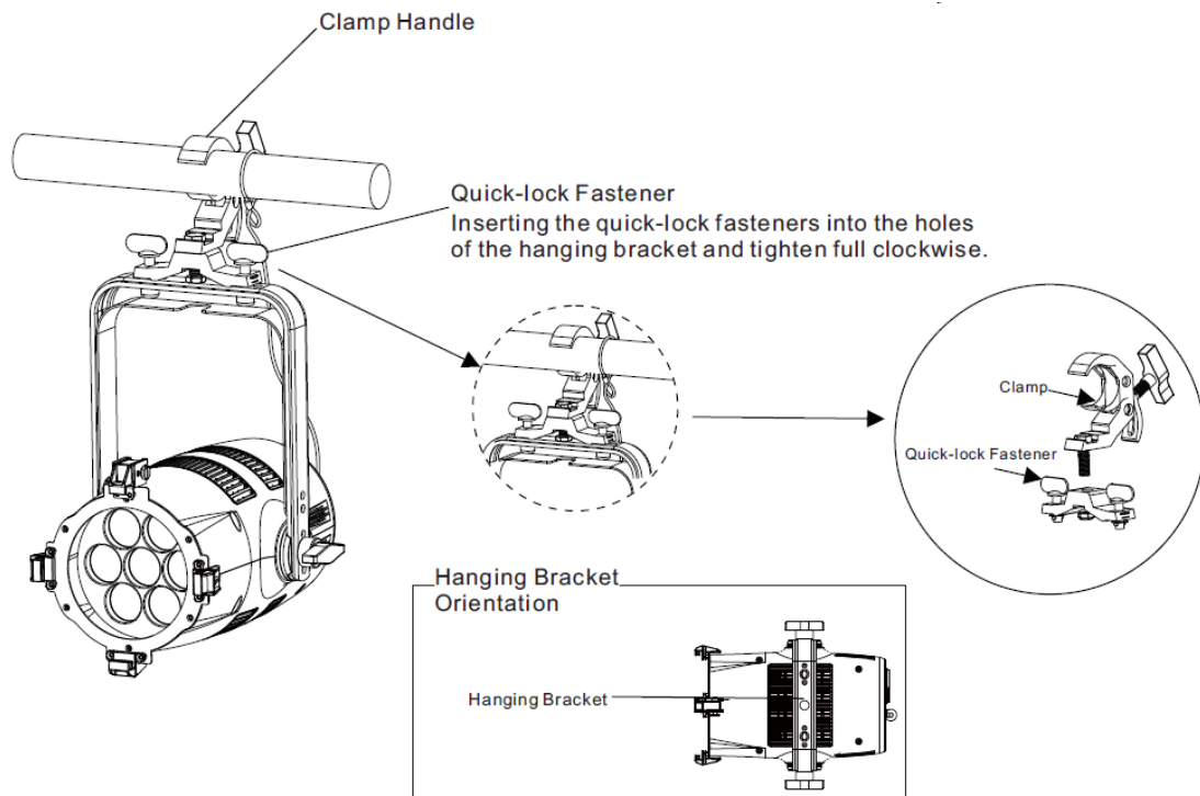
Figure 4: Installing Brackets on Luminaire Enclosure
