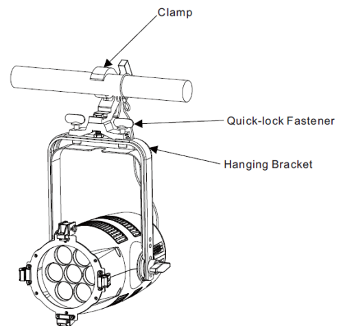
Figure 3: Quick-lock Fastener Installation
