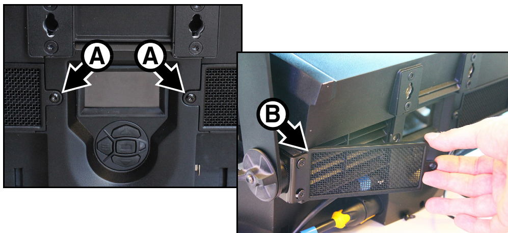
Figure 10: Removing air grills
